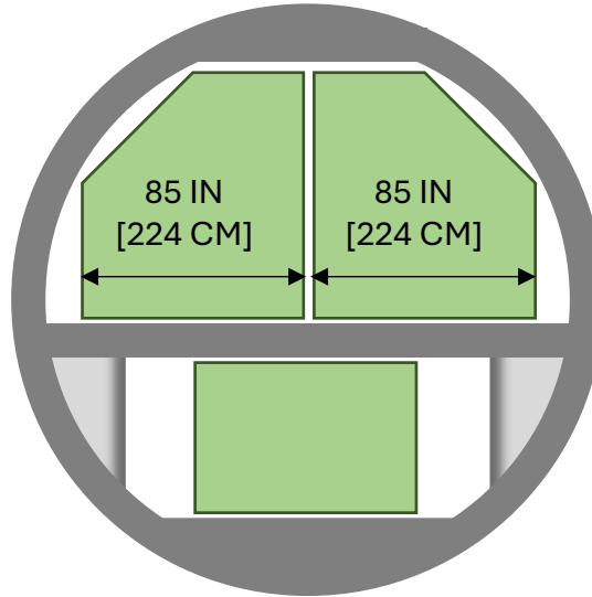
Longitudinal Main [SBS] Deck Loading
